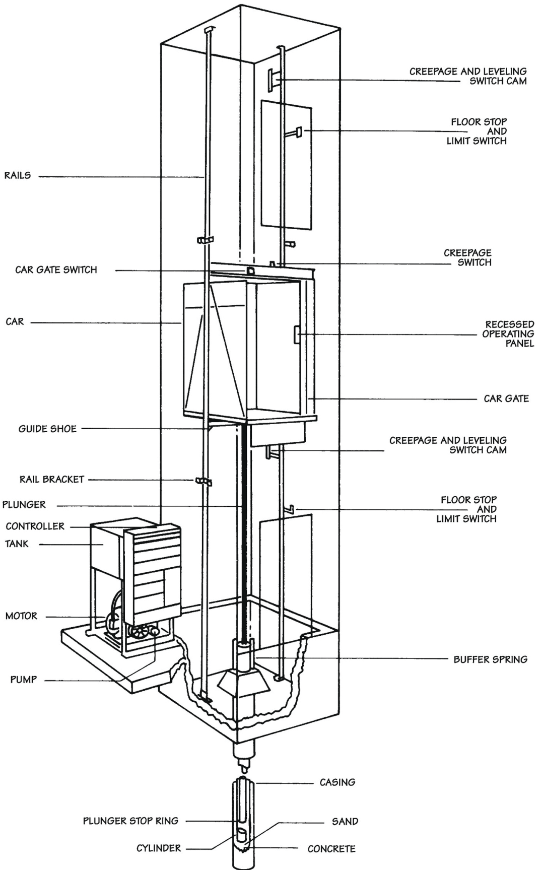
DIRECT PLUNGER
